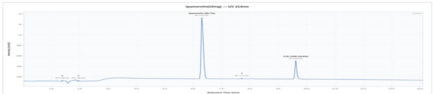
CJC-1295 / Ipamorelin (No DAC) 10mg - CIP0002: UV Chromatogram
