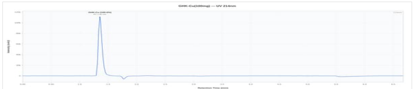
GHK-Cu 100mg - GHK0004: UV Chromatogram
