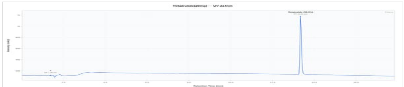
GLP-3 (RT) 20mg - RT0005: UV Chromatogram
