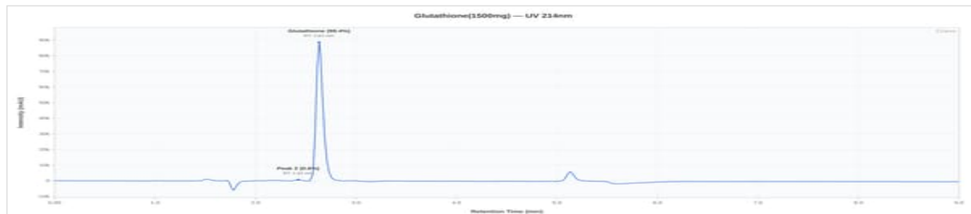
Glutathione 1500mg - GLT0002: UV Chromatogram
