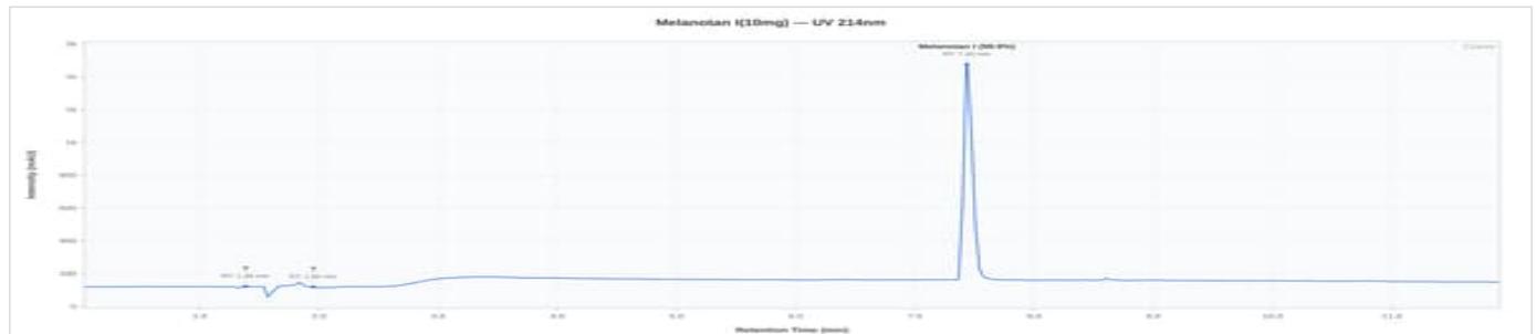
Melanotan I 10mg - MI0002: UV Chromatogram
